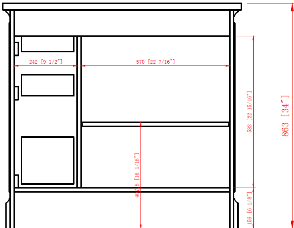
BACK VIEW
